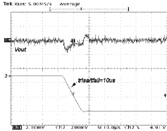
V_{CC} = 5.25 to 6.25V, I_{OUT} = 0.05A , C_{OUT} = 10\mu F , C_{IN} = 150nF (ESR=1Ω at 1KHz)
