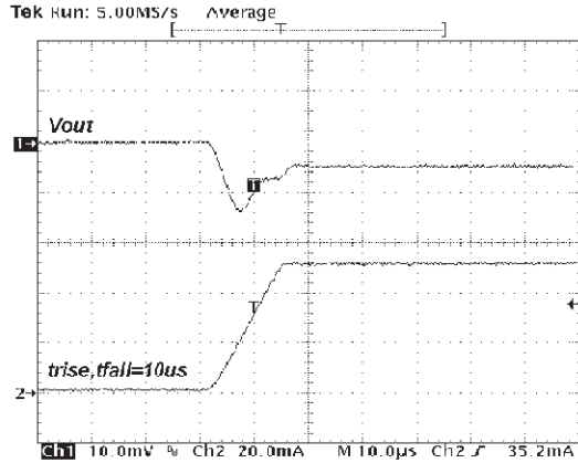
V_{CC} = 5V , I_{OUT} = 1 to 50mA, C_{OUT} = 10\mu F , C_{IN} = 150nF (ESR=1Ω at 1KHz)
