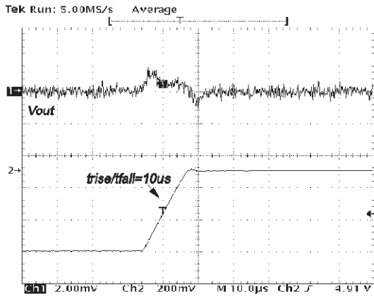
V_{CC} = 4.75 to 5.25V, I_{OUT} = 0.05A , C_{OUT} = 10\mu F , C_{IN} = 150nF (ESR=1Ω at 1KHz)
