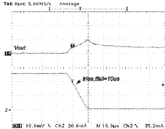
V_{CC} = 5V , I_{OUT} = 50 to 1mA, C_{OUT} = 10\mu F , C_{IN} = 150nF (ESR=1Ω at 1KHz)
